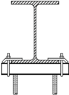
BEAM CLAMP
