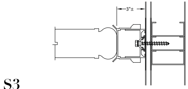
BULBSEAL MEETING JAMB - ALUMINUM
