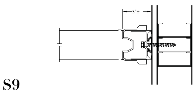
MEETING JAMB - ALUMINUM
