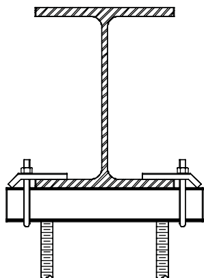
BEAM CLAMP
